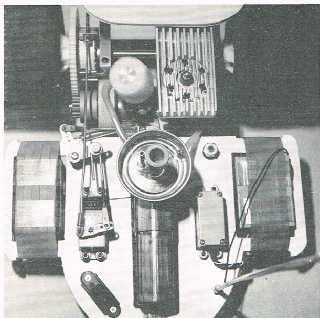
5 - RADIO INSTALLATION
