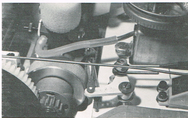
8 - THROTTLE BELLCRANK
