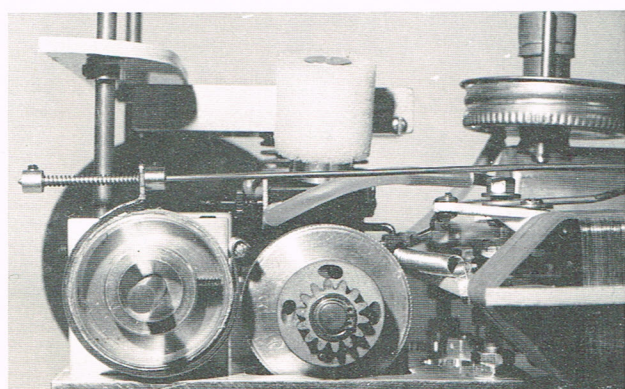
7 - BRAKE INSTALLATION - RC 100
