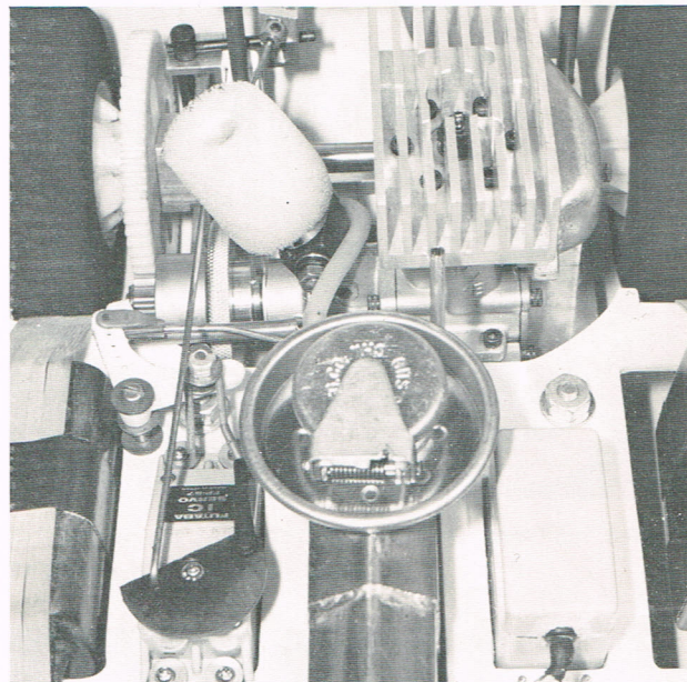
6 - CARB AND BRAKE LINKAGE
