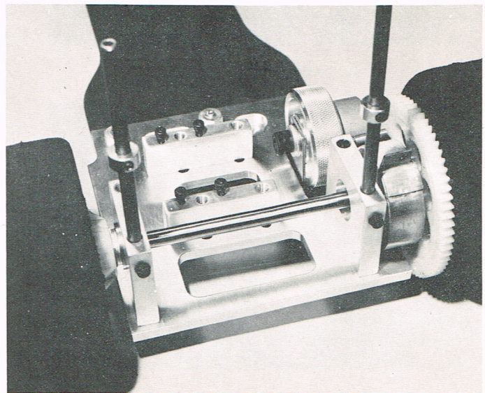
3 — BALL BEARING PILLOW BLOCKS
