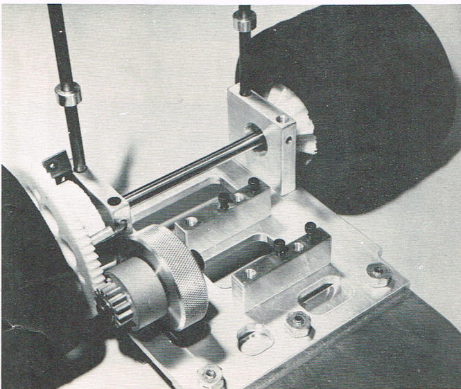
2 — ADJUSTABLE MOTOR MOUNTS
