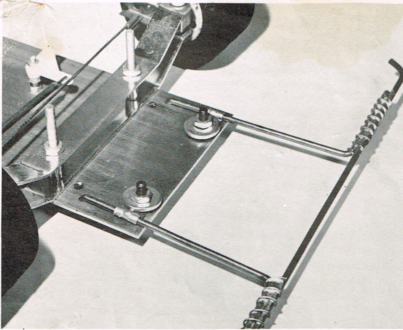
FRONT END ASSEMBLY
