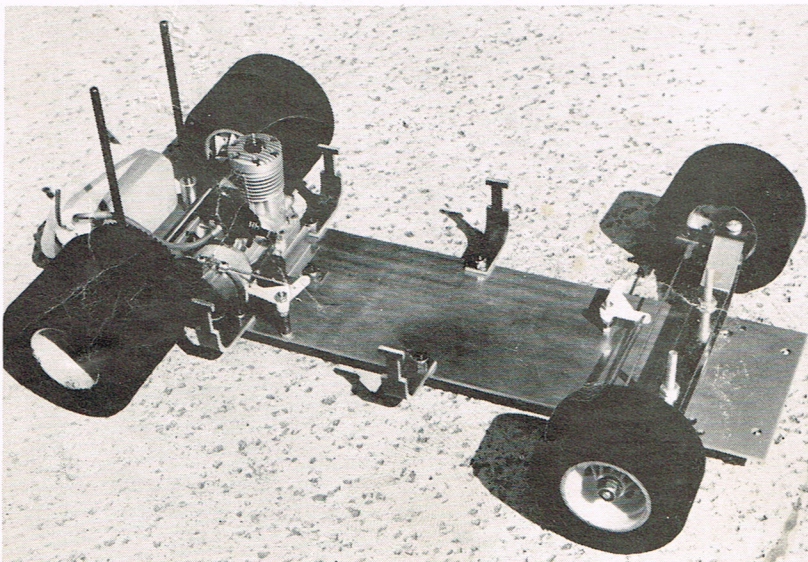
COMPLETED CAR (less radio)
