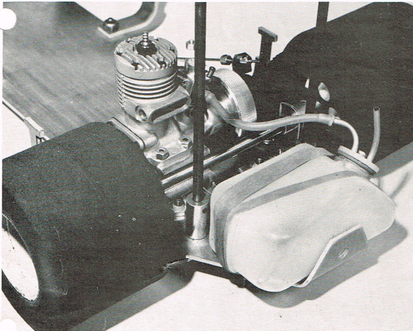
FUEL TANK INSTALLATION
