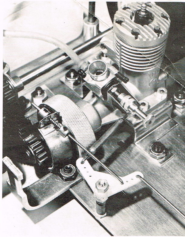
LINKAGE ASSEMBLY FOR STOCK VECO CARB & SELF-ENERGIZING TYPE BRAKE. Also shown is the four piece rear end/motor mount assembly used in the RC-2 kit.
