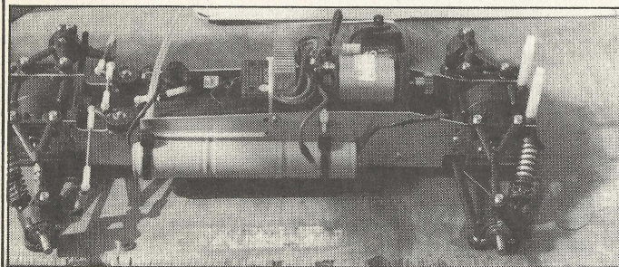
The SG/TAG 'Coyote' employs shaft drive between front and rear from an in-line motor. Ni-Cads are carried in two, three cell, sticks mounted either side of the chassis. Limited slip differentials feature front and rear.
