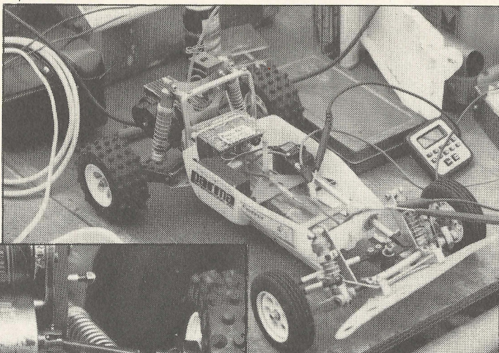
Above left: belt drive for the Benson's 'Scorpion' provided the answer to noisy and inefficient gear mesh. Left: John also produced their own rear trailing arms from steel to allay breakages in this area. Above: Associated 'RC10' shocks provided the damping and a lexan radio crate kept the weight down. Front anti-roll bar was also fitted.
