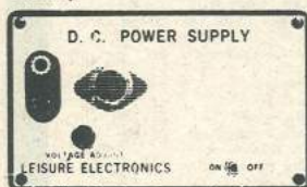
Leisure 110 DC Power Supply. A precise, adjustable power converter that delivers a healthy 1.4amps @ 12 volts of continuous current. Built-in short circuit and overload protection.
