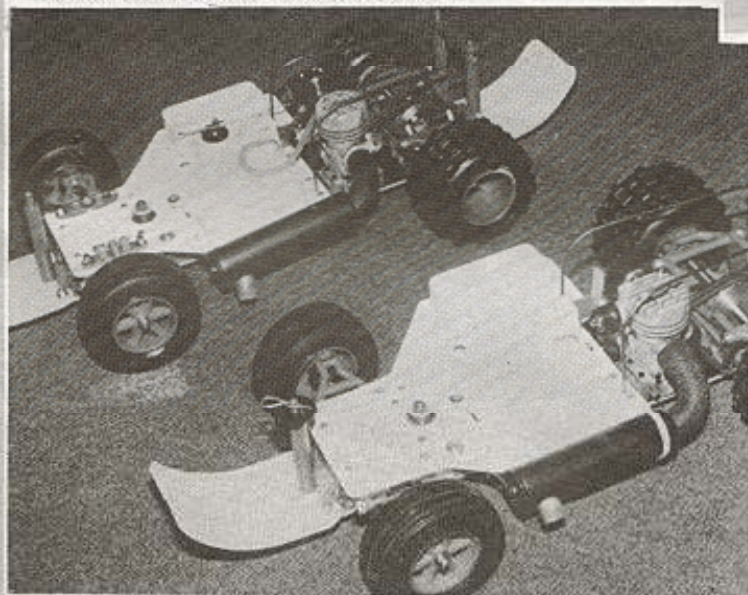
Above; latest in the Tamiya 'Competition Specials' range smart VW 'Golf'. Below left; PB Racing announced their new 'Mustang' at Nuremberg, basic version in front; full-house with shockers, anti-roll bar and differential in rear. Very robust, should be a good performer. Drive train shown below right.
