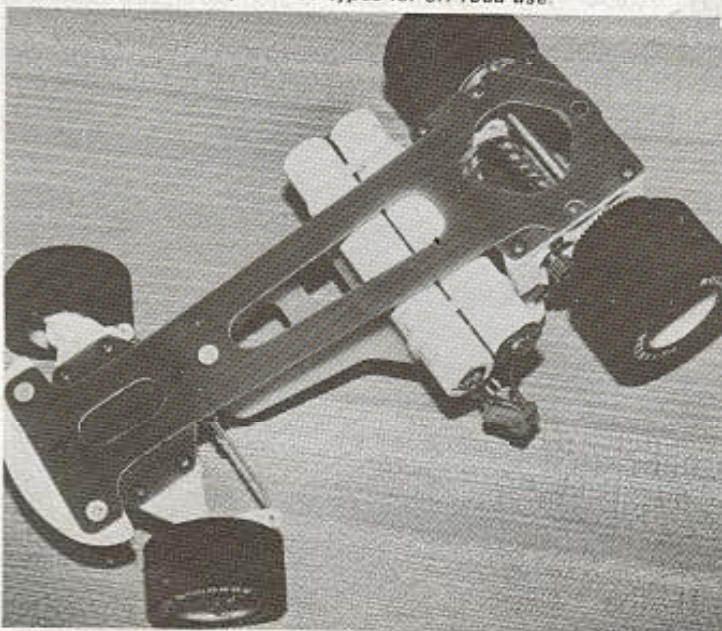
Above: latest version of Bolink 'Challenger' uses flexibly mounted front axles and rear motor pod. See below for underside view. Below right: AJS produce a wide range of foam tyres including these hefty treaded types for off-road use.
