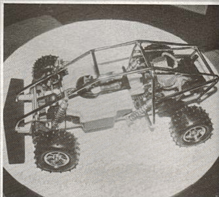
Above: Garbo buggy now with 4 wheel drive capability, very robust welded steel cage. Below: on-the-trackside tyre trimmer from Graupner runs from 12 volt battery.
