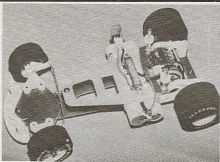
Above: latest version of Bolink 'Challenger' uses flexibly mounted front axles and rear motor pod. See below for underside view. Below right: AJS produce a wide range of foam tyres including these hefty treaded types for off-road use.
