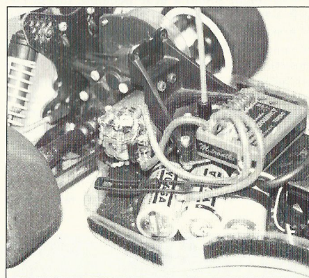
The cells are positioned in such a way that the original Cougar 2000 undertray and bodyshell (slight trimming is needed at the rear) can be used. The front two cells are very close together, the intention being to maintain a low polar moment of inertia, whilst the heavy items on the car (the motor and cells) are closely grouped for beautifully balanced weight distribution.
