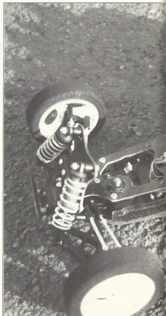
Look Ma, no motor! The lack of a motor at the rear, allied with the Fab 2000's handling, often misleads spectators into thinking it's actually a 4wd car!
