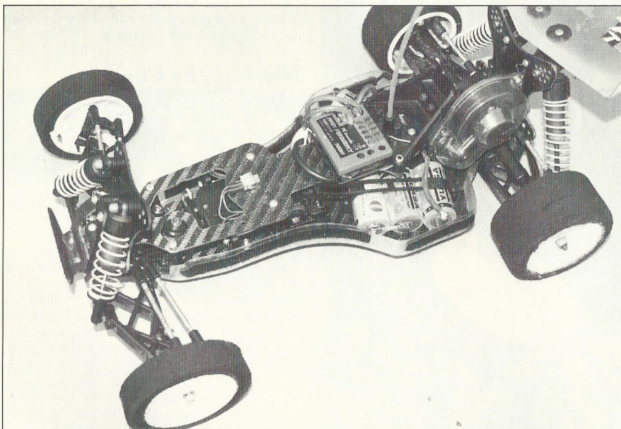
As the Fab 2000 is based around the well proven Schumacher Cougar transmission and running gear, there need be no fear of not being able to source spare parts at race meetings. It all looks as if it was designed to be like this right from the start, and is really professional in its appearance. The latest Schumacher 'SACS MK2' front end works very well on the Fab 2000, and gives superb steering into and throughout a corner.
