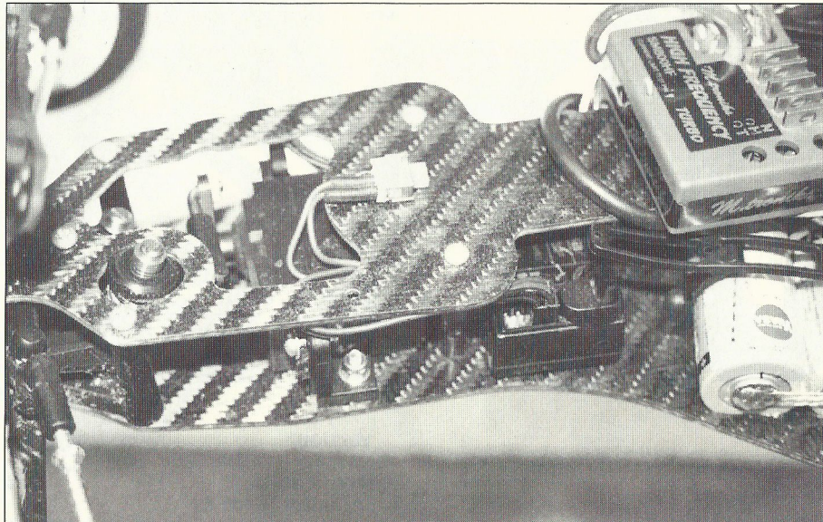
The top deck is braced mid-way along the chassis by one of the original Schumacher moulded 'gates', situated between the receiver and the steering servo. Space for radio gear is slightly limited, but it all goes in eventually!
